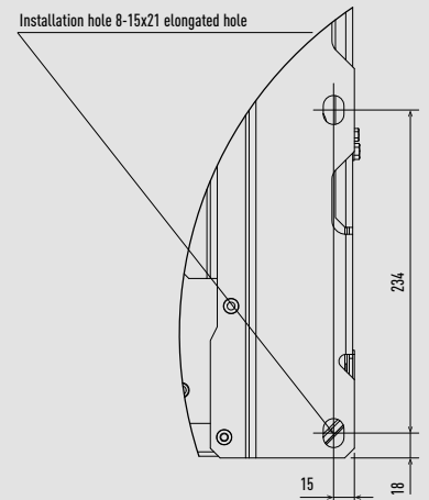
View D
