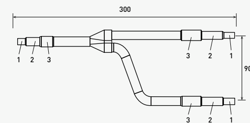
Liquid piping
