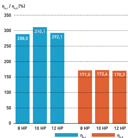
1) 12 HP model compared to the equivalent conventional R410A ECOi EX model. 2) 8 and 10 HP models.
