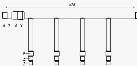
Size of connection point on each part (shown are inside diameters of piping)
