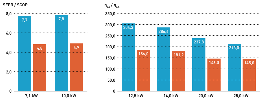
PZH4 Series seasonal performance.
