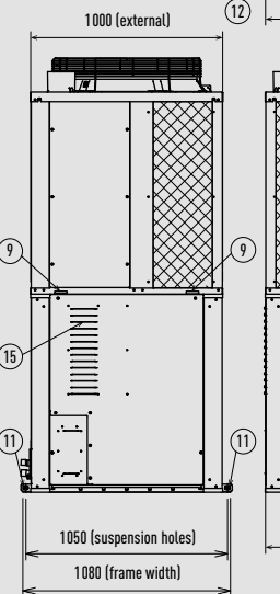
Left view
