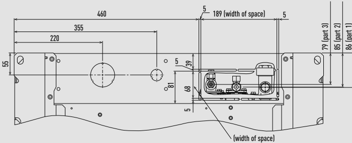
View E
