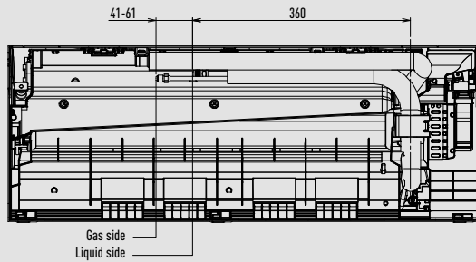
Rear view
